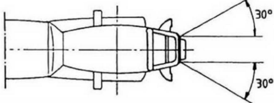
ANGOLO DI VISIBILITA' GEOMETRICA (DIEDRO CON SPIGOLO PRATICAMENTE VERTICALE) ANGLE OF GEOMETRIC VISIBILITY (DIEDRAL WITH PERCEPTIBLY VERTICAL EDGE)
